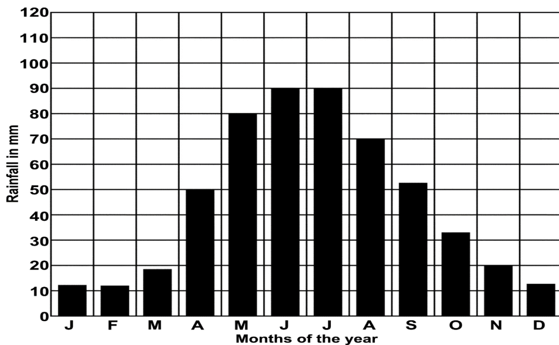
Annual rainfall for Cape Town
